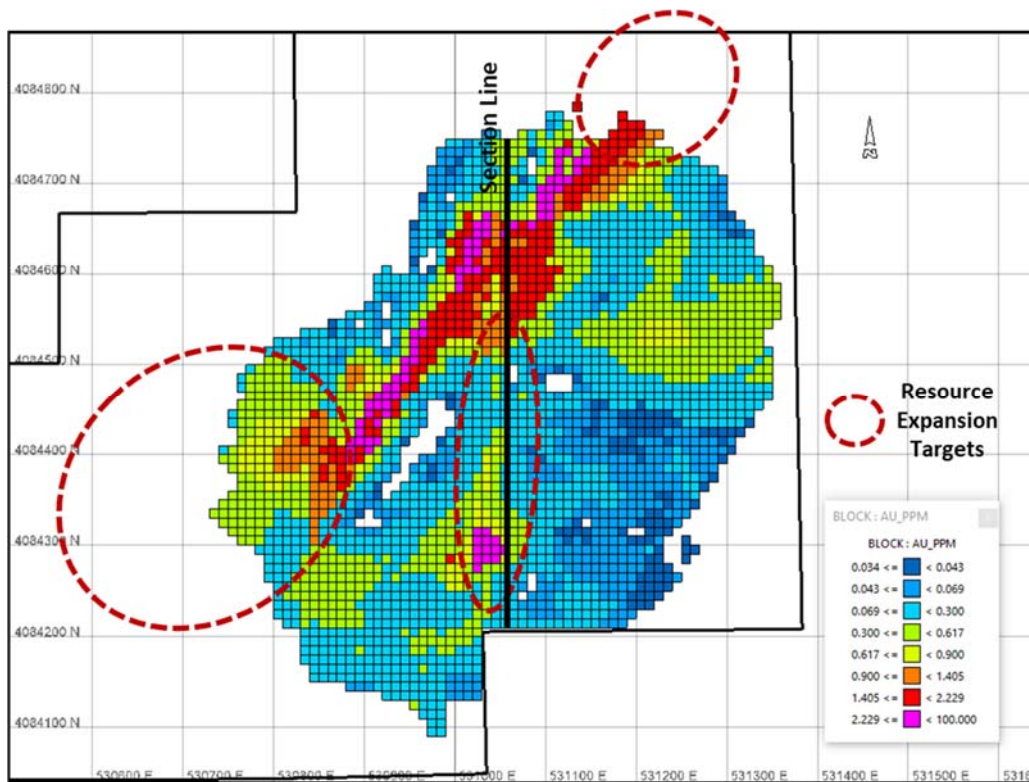
Figure 4. Plan View of Mother Lode resource block model at 970 m elevation (UTm NAD27 Z11)
